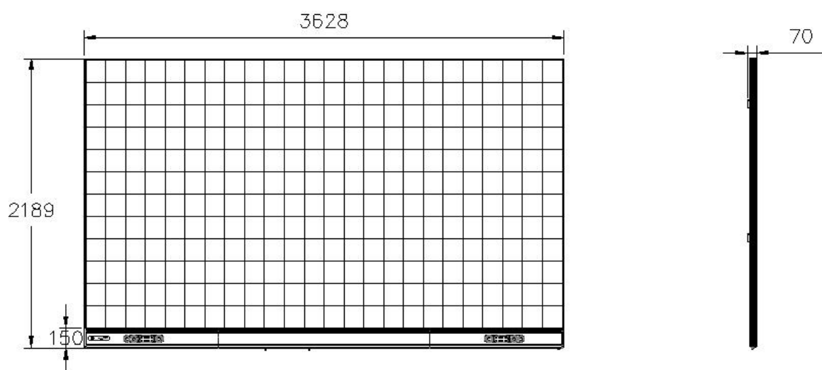
163" Wall-Mount Installation Dimensions
