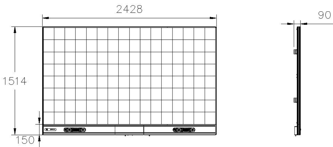
108" Wall-Mount Installation Dimensions
