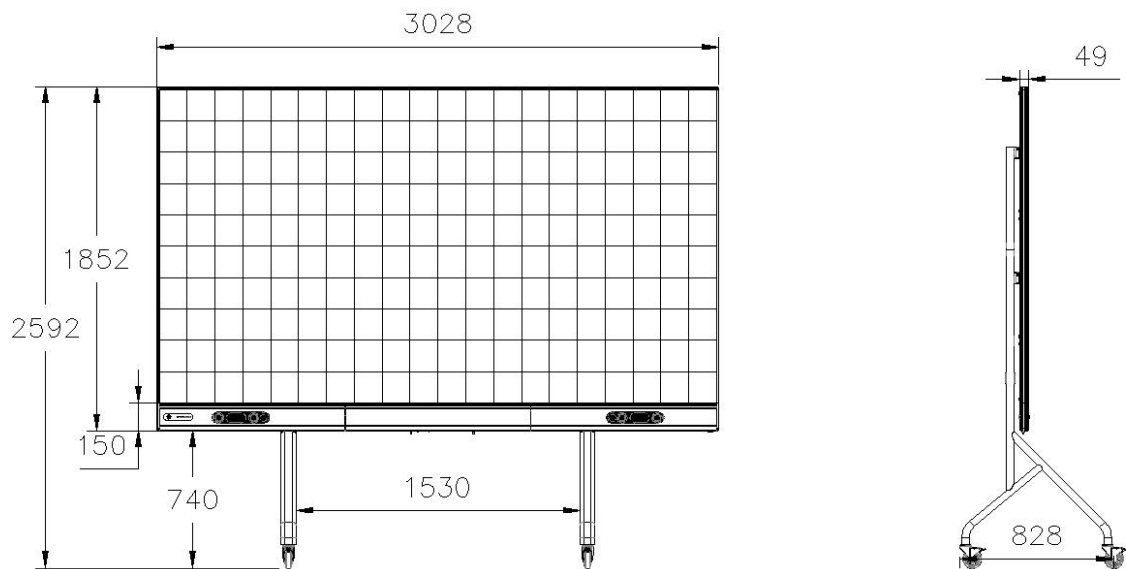
135" Mobile stand Installation Dimensions
