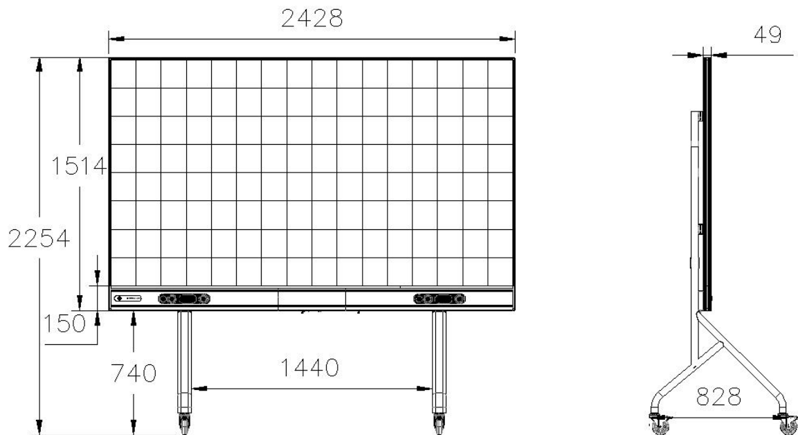
108" Mobile stand Installation Dimensions
