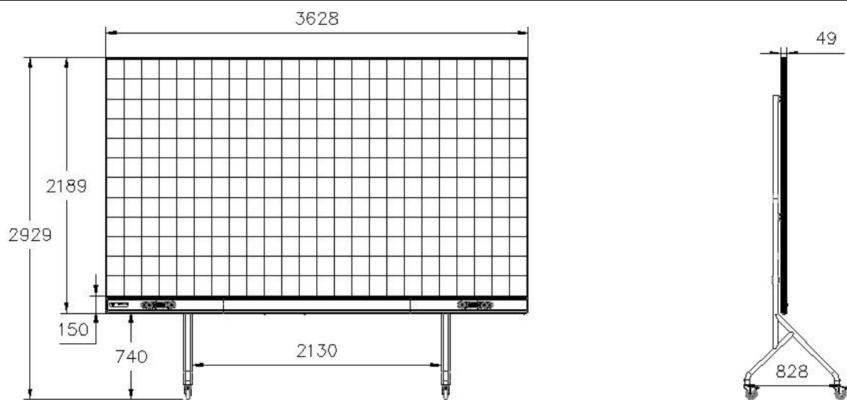
163" Mobile stand Installation Dimensions
